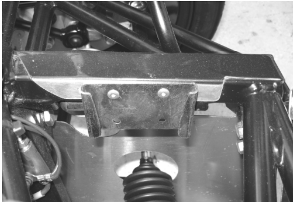
Fig 14 Breather bottle mounting Bracket
