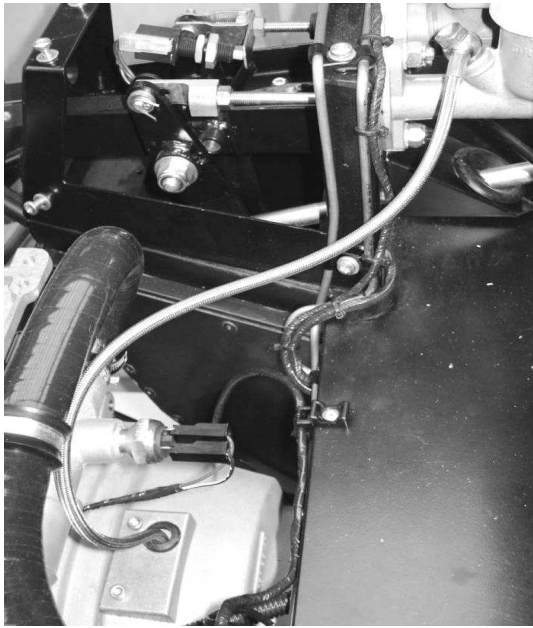
Fig 9 Clutch hydraulic hose
