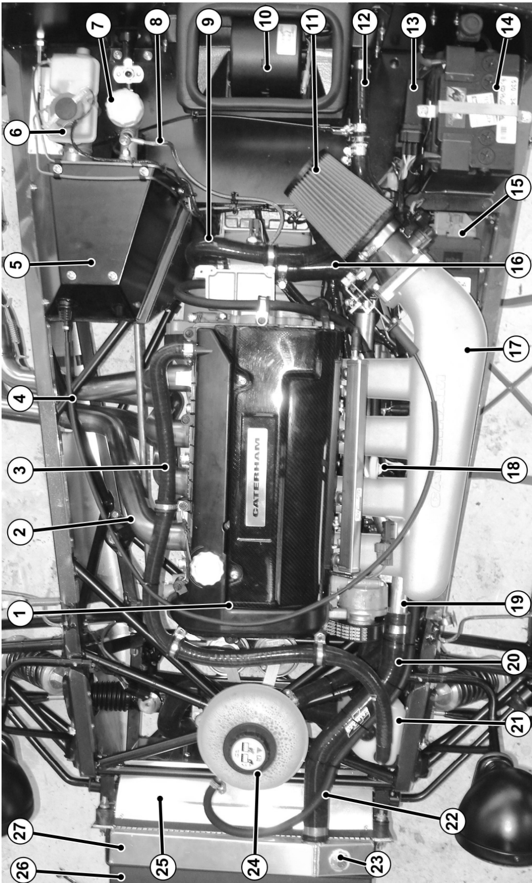
Fig 30 R400 Engine bay overview
