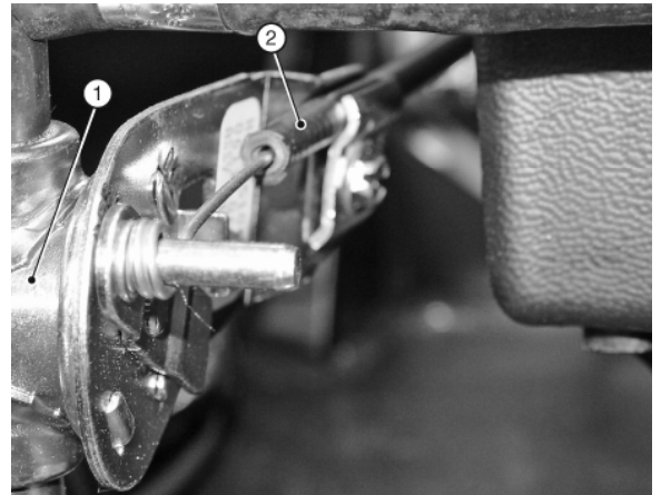
Fig 26 Heater control cable
