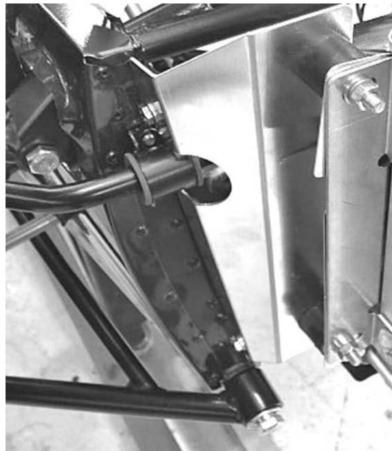
Fig 19 SV radiator arrangement
